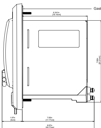
Nexus® 1262/1272 Switchboard Case Side View
