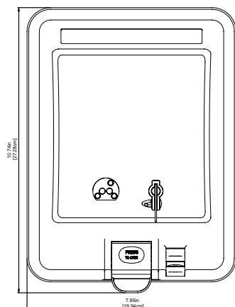
Nexus® 1262/1272 Switchboard Case Front View
