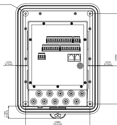
Nexus® 1262/1272 Switchboard Case Back View
